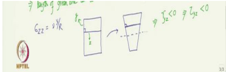
Figure 10: Undeformed and deformed cross-sections considering the effects of \epsilon_{zz} only.
