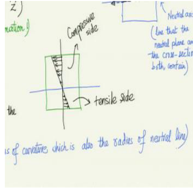
Figure 6: Variation in \sigma_{xx} along the beam's height.
