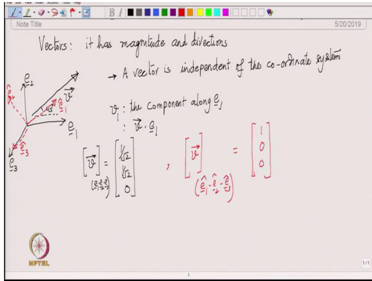
Figure 1: A vector \vec{v} observed from two different coordinate systems
