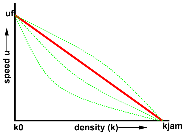
Figure 31:4: Speed-density diagram
