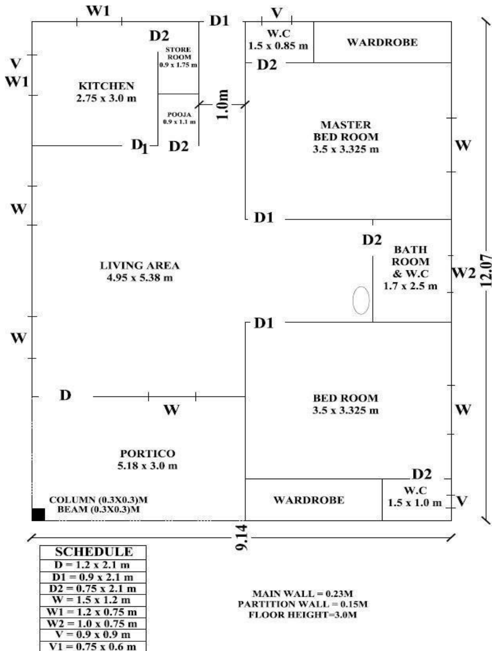
Q.no.3.1:-LINE DIAGRAM OF SINGLE STOREY RESIDENTIAL BUILDING
